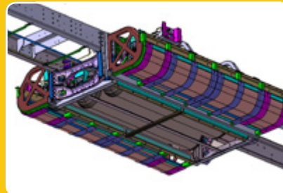
Four CNG tanks (60 diesel gallon equivalent).
